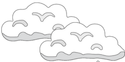
clouds
