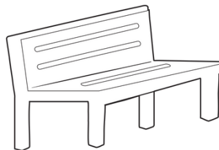
bench
