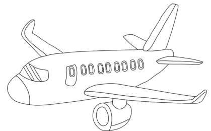
airplane
