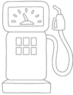
gas station
