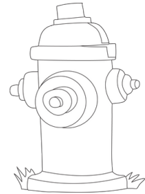
fire hydrant
