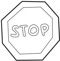
stop sign
