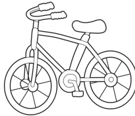
bike
